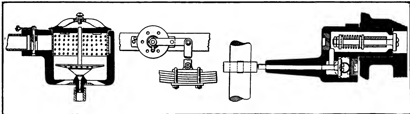
Fig. 1—Mallo carbureter.
